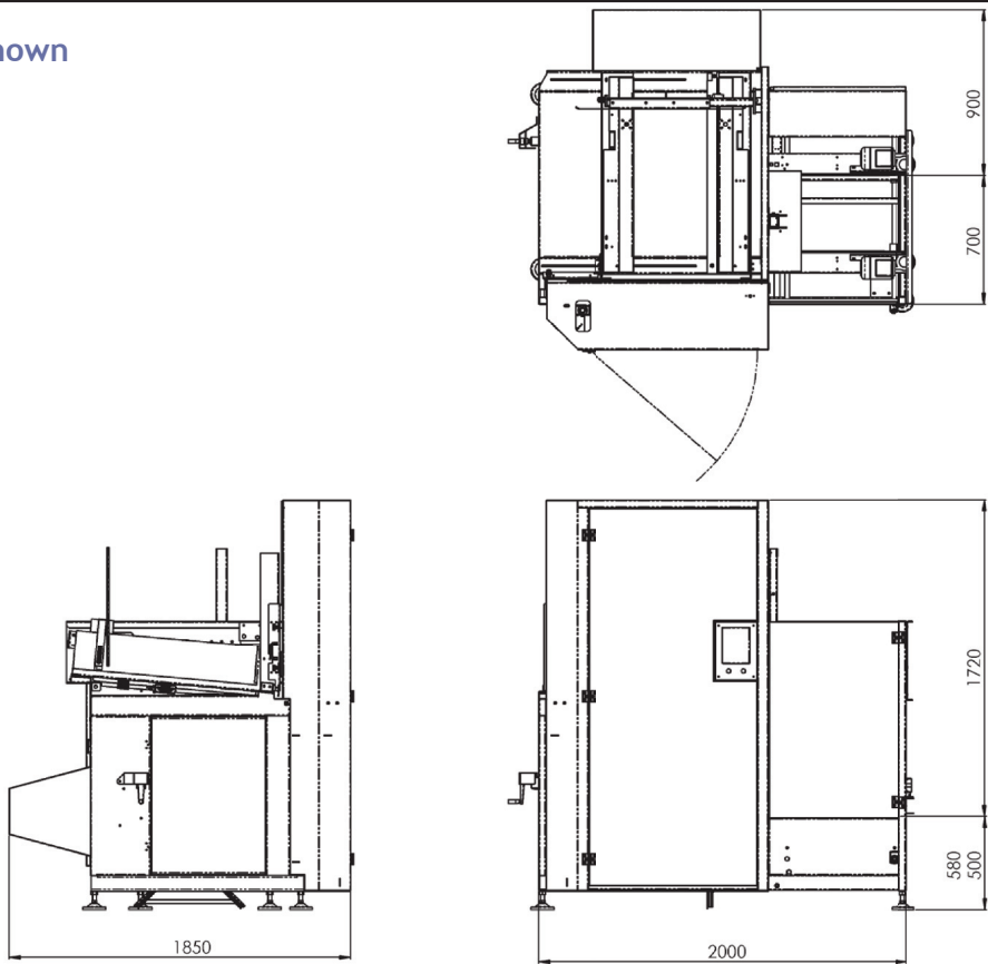
Case Dimensions (mm).
